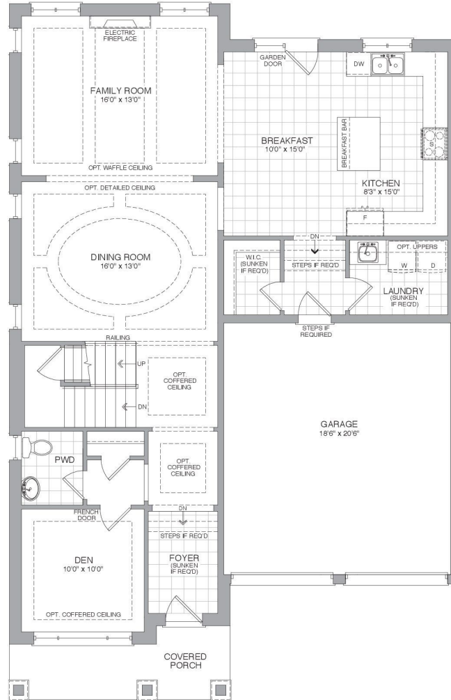
GROUND FLOOR ELEV C1
