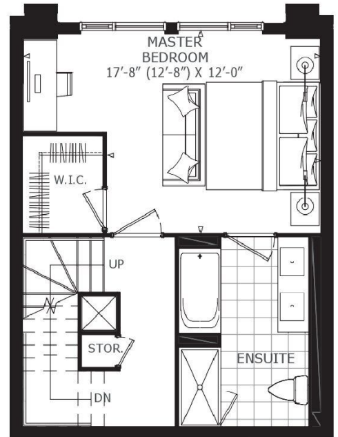
FLOOR 2 (OPTION 2)
