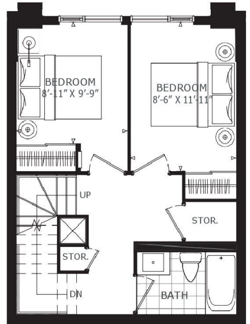
FLOOR 2 (OPTION 1)
